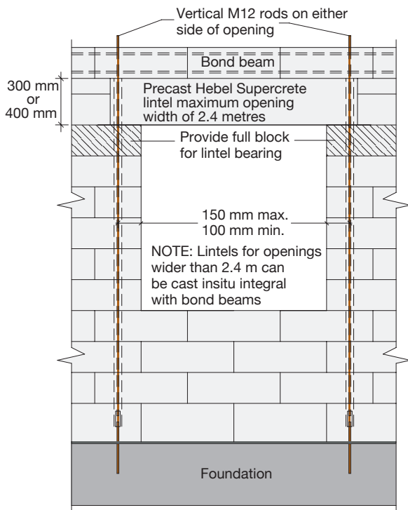
Detail 4. Typical Lintel Detail
