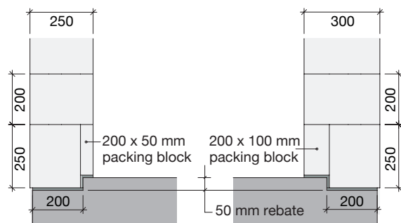
Detail 5. First Course Detail for Varying Wall Thickness
